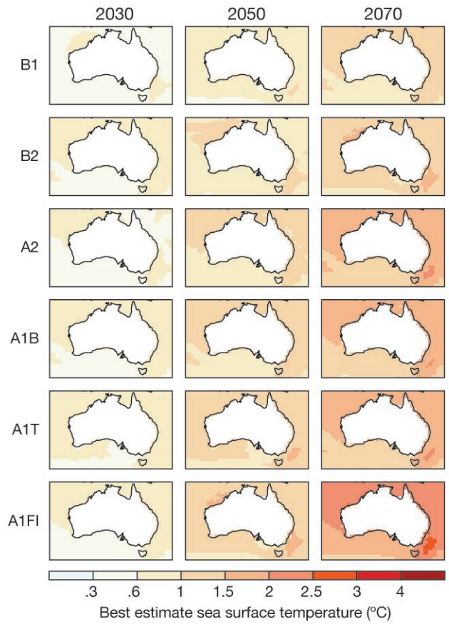
Figure S25: Best estimate, 10th percentile and 90th percentile annual sea surface temperature change (°C) for 2030, 2050 and 2070 and six SRES emission scenarios.
